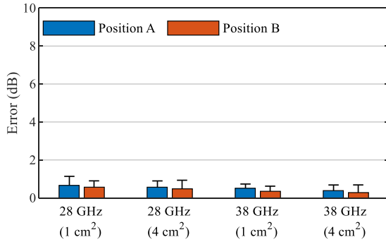
Fig. 15. The mean and maximum values of the reconstruction errors for the 1 cm 2 and 4 cm 2 psaPD at 28 GHz and the 1 cm 2 and 4 cm 2 psaPD at 38 GHz reconstructed from the simulated IF data when the origin is set at different positions. Each bar contains 124 samples from different combinations of antenna (Ant 1–4) and evaluation distance (from d = 5 mm to d = 35 mm with 1 mm step).
