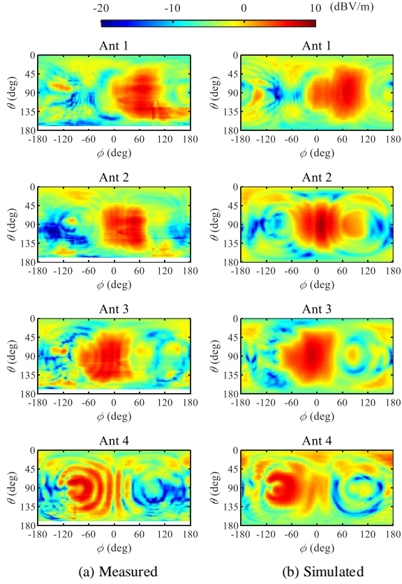
Fig. 3. (a) The measured and (b) simulated |E| distributions over \Sigma_M , a sphere with radius of 450 mm, in the IF region of Ant 1–Ant 4 at 28 GHz. The input power is normalized to 5 dBm.
