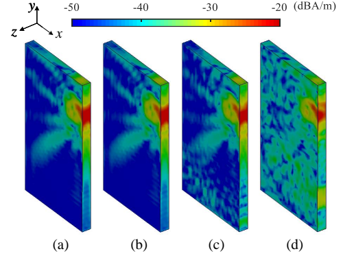
Fig. 9. |J_{\text{eq}}| distributions reconstructed from the simulated IF data of Ant 3 at 28 GHz with the angular resolution of (a) \Delta\alpha = 2^\circ , (b) \Delta\alpha = 4^\circ , (c) \Delta\alpha = 6^\circ , and (d) \Delta\alpha = 8^\circ .
