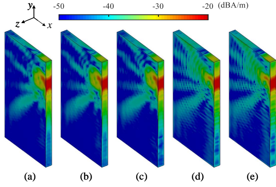
Fig. 11. |J_{eq}| distributions reconstructed from the simulated IF data of Ant 3 at 28 GHz with the phase noise level of (a) \sigma = 0^\circ , (b) \sigma = 5^\circ , (c) \sigma = 10^\circ , (d) \sigma = 15^\circ , and (e) \sigma = 20^\circ .
