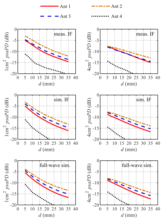
Fig. 8. The 1 \text{ cm}^2 (left column) and 4 \text{ cm}^2 (right column) psaPD at 38 GHz as the evaluation distance varies for Ant 1–Ant 4. The values are normalized with 20 \text{ W/m}^2 .
