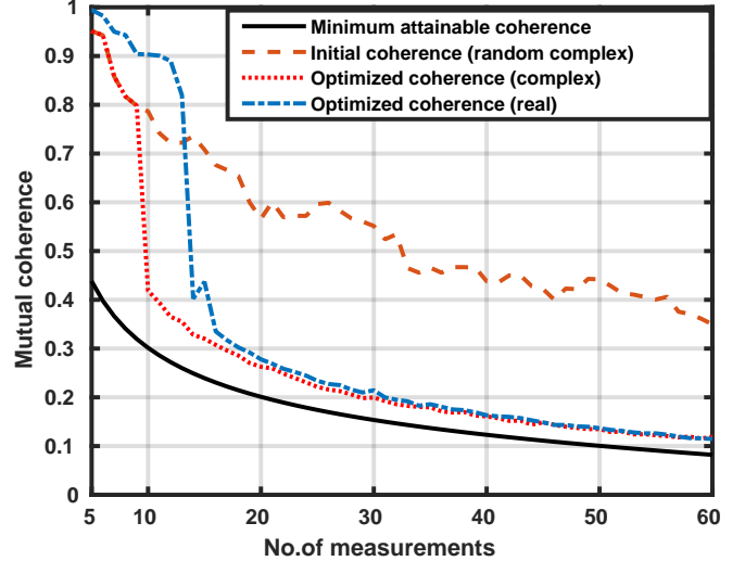
Fig. 3. Mutual coherence values for M \times 100 matrices for random, optimized, and real sensing matrices. The amplitude and phase of every matrix element has been quantized to 6 bits each in the case of complex measurements, whereas this quantization is to 6 bits amplitude and 1 bit phase (i.e. a \pm sign), in the case of real measurements.
