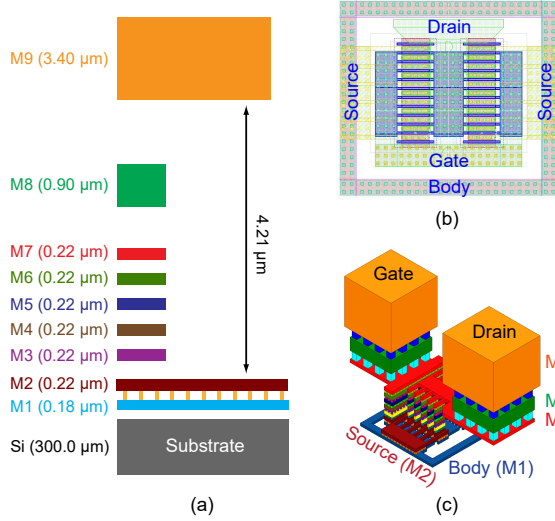
Figure 7. (a) Stack-up of the 65-nm CMOS technology. (b) Layout of the 16-μm NMOS transistor. (c) Interconnect setup used for connecting to the transistor.
