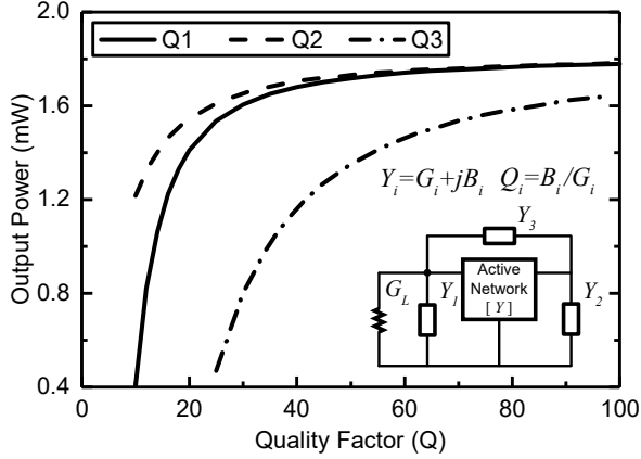
Figure 6. Simulated oscillator output power with respect to the component Q of the embedding network. An NMOS transistor ( W/L = 16 \mu\text{m}/60 \text{ nm} ) is used as the active device in an oscillator topology given by the inset. Simulation is done at 215 GHz.
