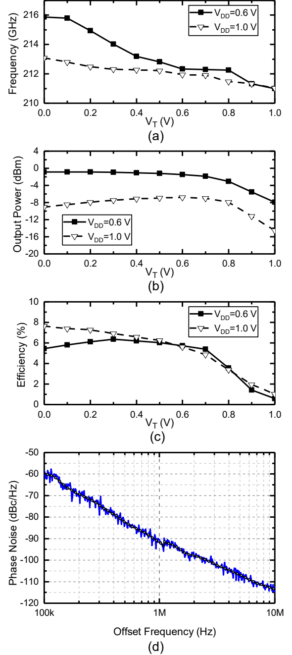
Figure 15. Measured output frequency (a), output power (b) and dc-to-RF efficiency (c) of the 213 GHz fundamental VCO with respect to the bulk tuning voltage ( V_T ), and measured phase noise with respect to offset frequency (d).
