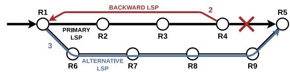
Fig. 14: Illustration of the underlying idea of the improved protection methods described in [112], [137].
