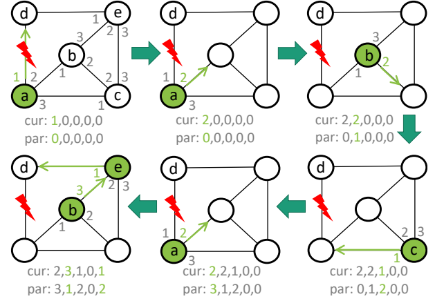
Fig. 29: Depth-first search example.
