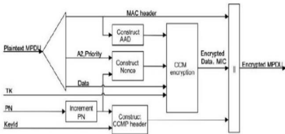
Figure 9: CCMP Encryption [34]
