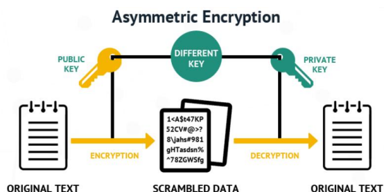
Figure 2: Asymmetric Encryption [5]
