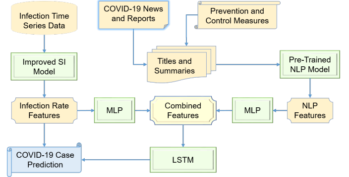
Fig. 3. An AI-based approach to COVID-19 prediction that combines traditional epidemic SI model, NLP and machine learning tools as introduced in [42]. A pre-trained NLP model is used to extract NLP features from text data, i.e. the pandemic news, reports, prevention and control measures. These features are integrated with infection rate features obtained from the SI model via multilayer perceptron (MLP) networks before being fed into LSTM model for COVID-19 case modelling and prediction.
