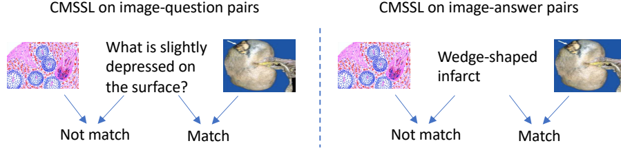
Figure 3: Cross-modal self-supervised learning.
