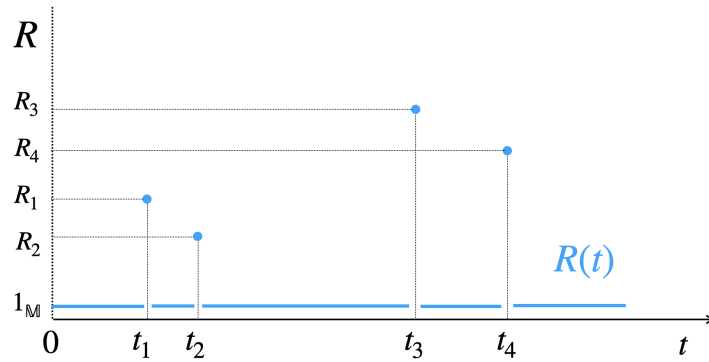
Fig. 3. Redistribution function.
