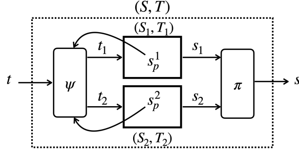
Fig. 14. Weak parallel decomposition.
