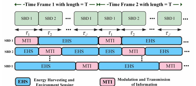
Fig. 8: The TDD frame for EHS and MTI modes in TDMA transmission information model
